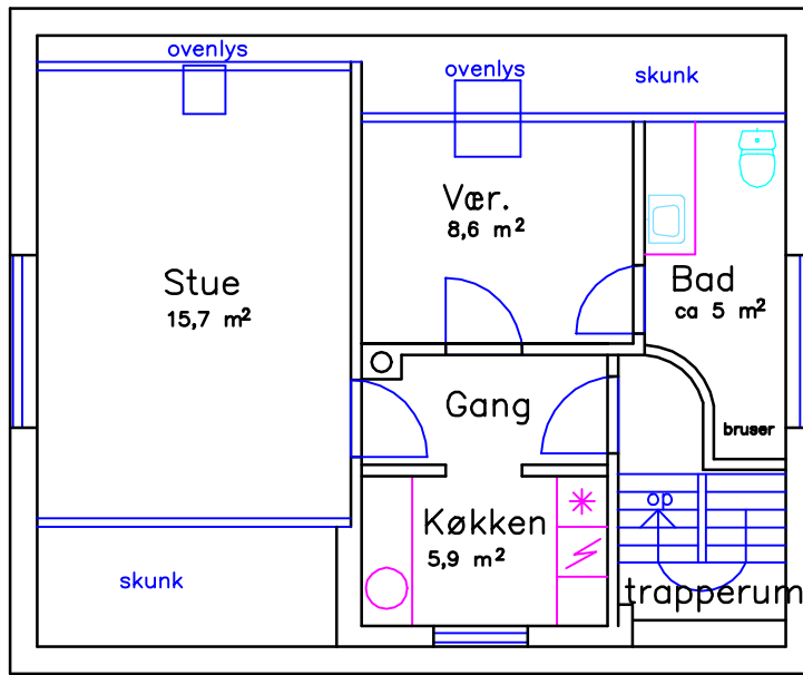
1.sals plan
